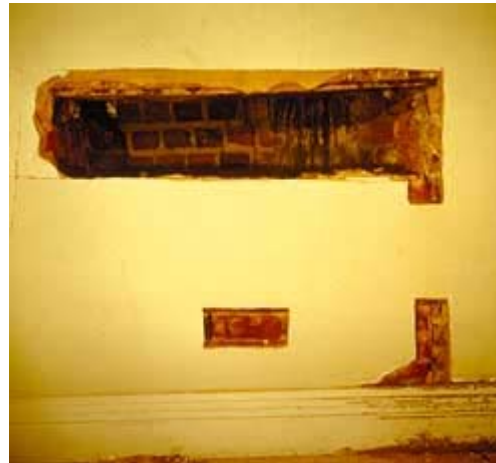
Exploratory testing was used to verify the location of an abandoned fireplace. Plaster and brick were carefully documented and removed to determine the fireplace's type, size, and location. Photo: Travis C. McDonald, Jr.
